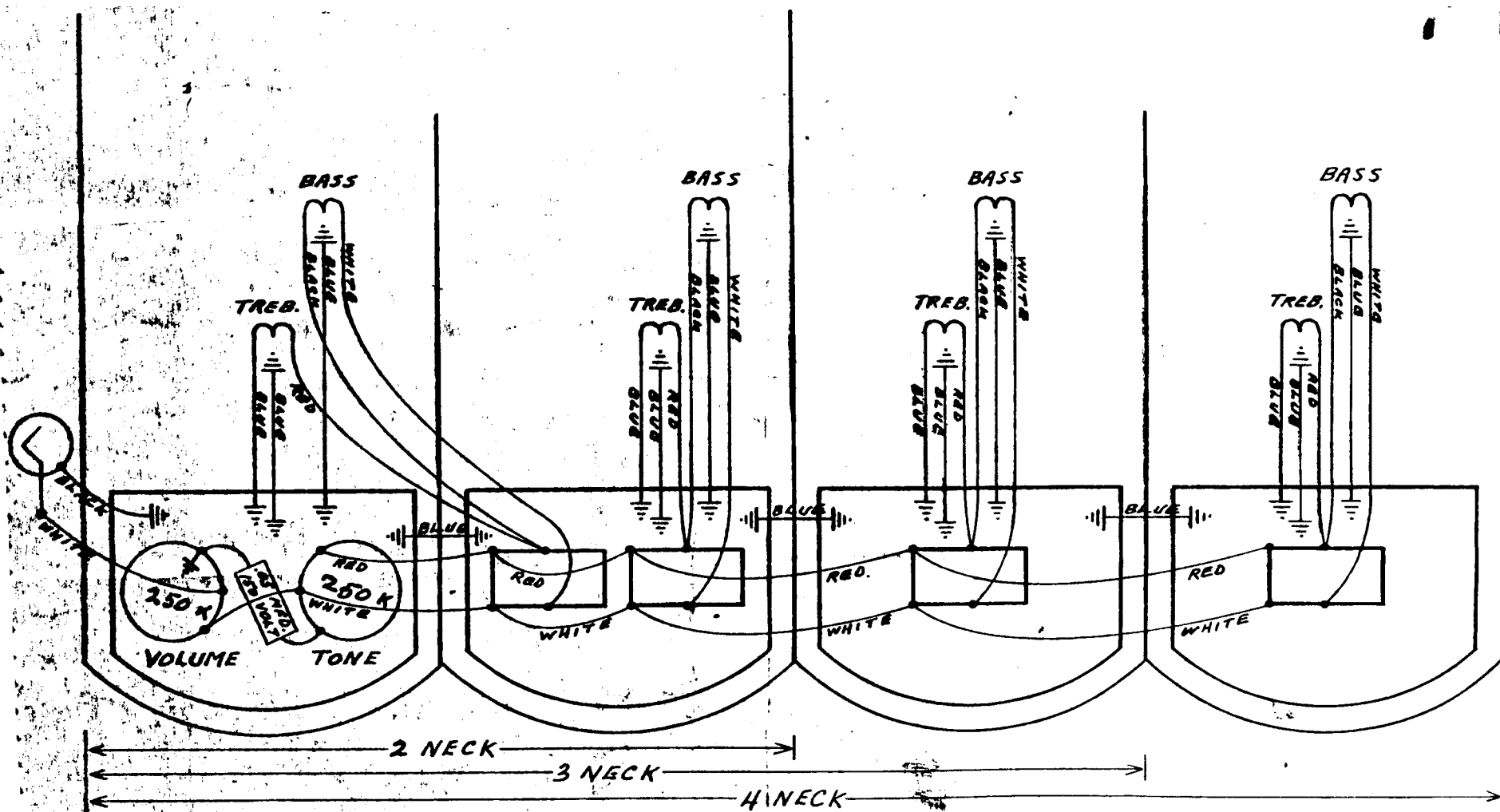
WIRING INSTALLATION - TOP VIEW OF INSTRUMENT SHOWN
